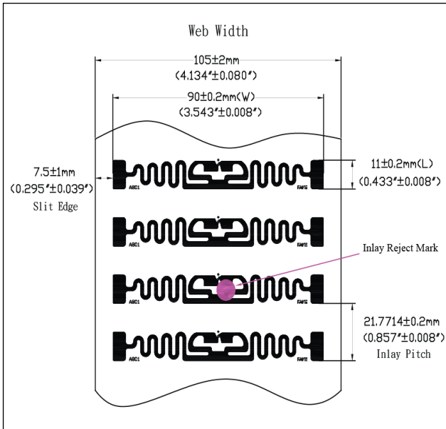
A801 Dry Inlay (IC Face Up)
