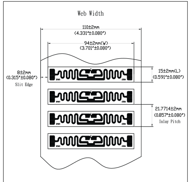
A801 Wet Inlay (IC Face Down)
