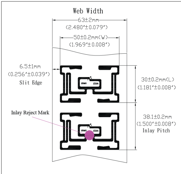
A601 Dry Inlay (IC Face Up)
