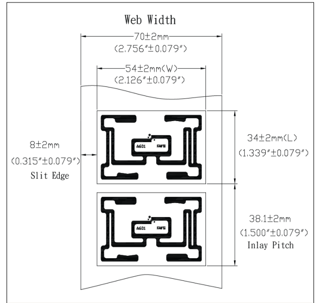
A601 Wet Inlay (IC Face Down)
